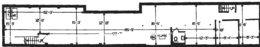
LOWER LEVEL
